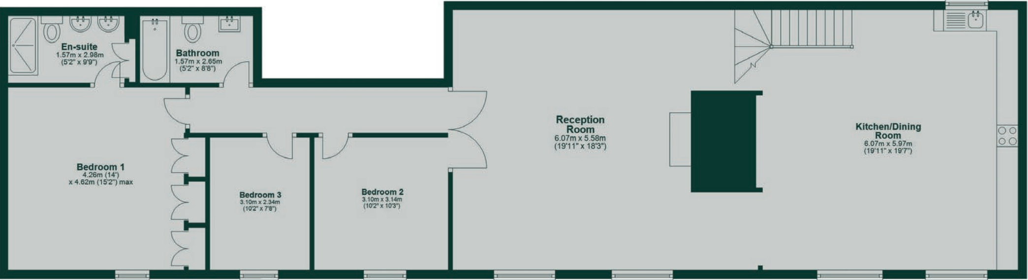
First Floor Approx. 134.1 sq. metres (1443.9 sq. feet)
